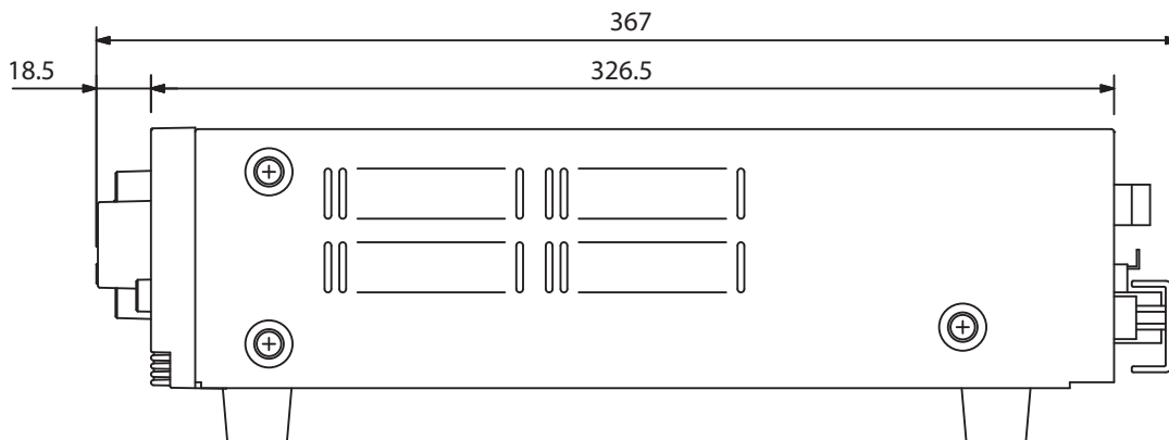
Side View
